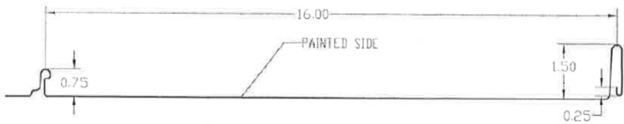
FIGURE 2—511 UNIVERSAL STANDING SEAM STEEL ROOF PANELS
