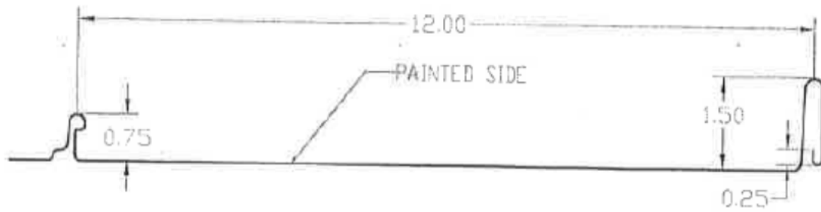
FIGURE 1—501 UNIVERSAL STANDING SEAM STEEL ROOF PANELS
